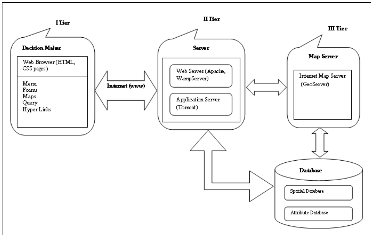
Fig. 2 Web GIS based Decision Support System Architecture
