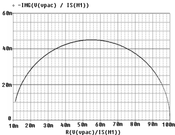
Fig. 4 Representation of the Nyquist plot simulation
