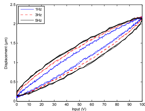
Fig. 2 Hysteretic behavior of the PSA-driven system
