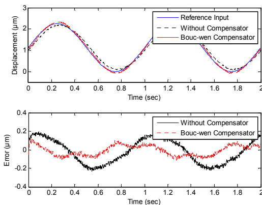
Fig. 6 1-Hz tracking by stand-alone Bouc-Wen feedforward control
