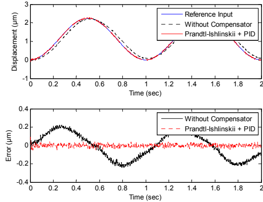
Fig. 9 1-Hz tracking by inverse P-I feedforward-feedback control
