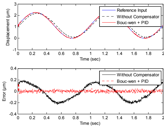
Fig. 7 1-Hz tracking by Bouc-Wen feedforward-feedback control
