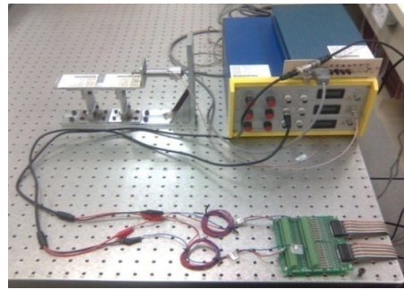
Fig. 1 A photograph illustrating the experimental set-up
