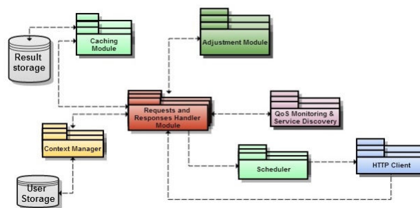
Fig. 3 Middleware General Architecture
