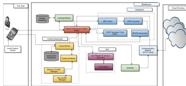
Fig. 4 Middleware Detailed Architecture
