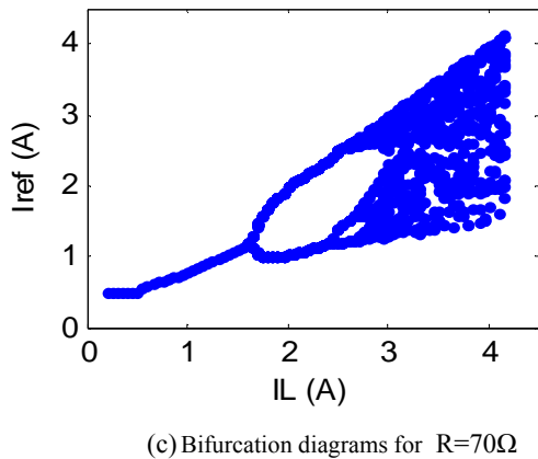
Fig. 4 Period-doubling cascade interrupted by a border collision Dimensionless parameter that is relevant to this bifurcation is R. From (a) to (d), the resistor gradually changes from a small value to a large value
