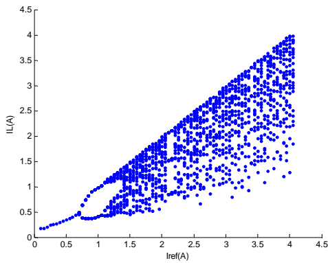
Fig. 3 Bifurcation diagrams from a current-mode controlled Boost converter
