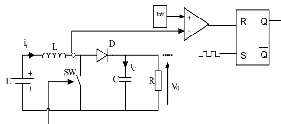
Fig. 1 Schematic diagram of the Boost converter under current-mode control
