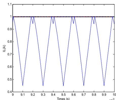
Reponses of the inductor current i_L
