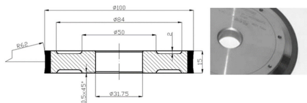
Fig. 6 The grinding wheel 1FF1V 100 – 15 – R62 – 31.75 D126 Ni [9]
