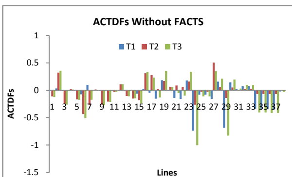
Fig. 1 ACTDFs without FACTS
