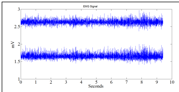
Fig. 6 EMG signal
