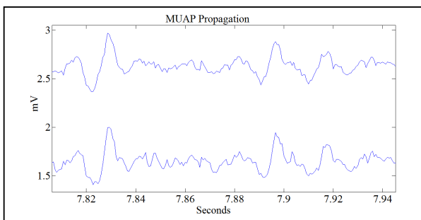
Fig. 7 Two differential channels of a 0.15s window of a S-EMG signal. It is possible to see the MUAPs traveling from the left to the right. The Inter Electrode Distance is 20mm
