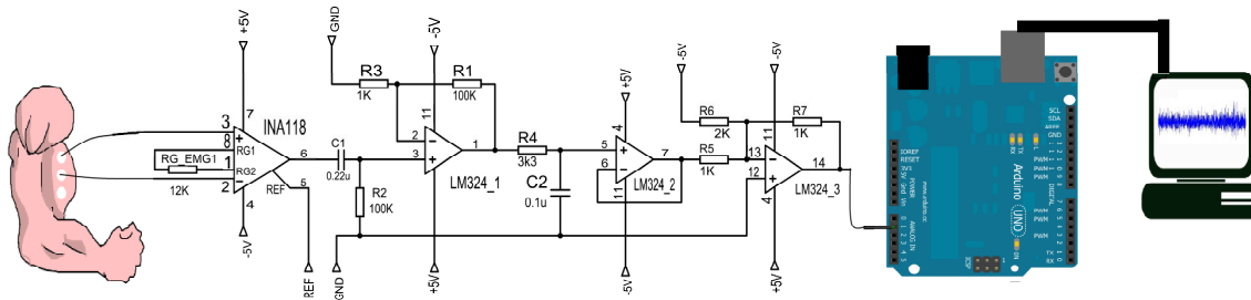
Fig. 1 Electrode configuration (left) followed by the amplification (500x) and band-pass filter (10-500Hz) circuit, the output of this circuit is digitalized by the Arduino microcontroller that export the result to a computer
