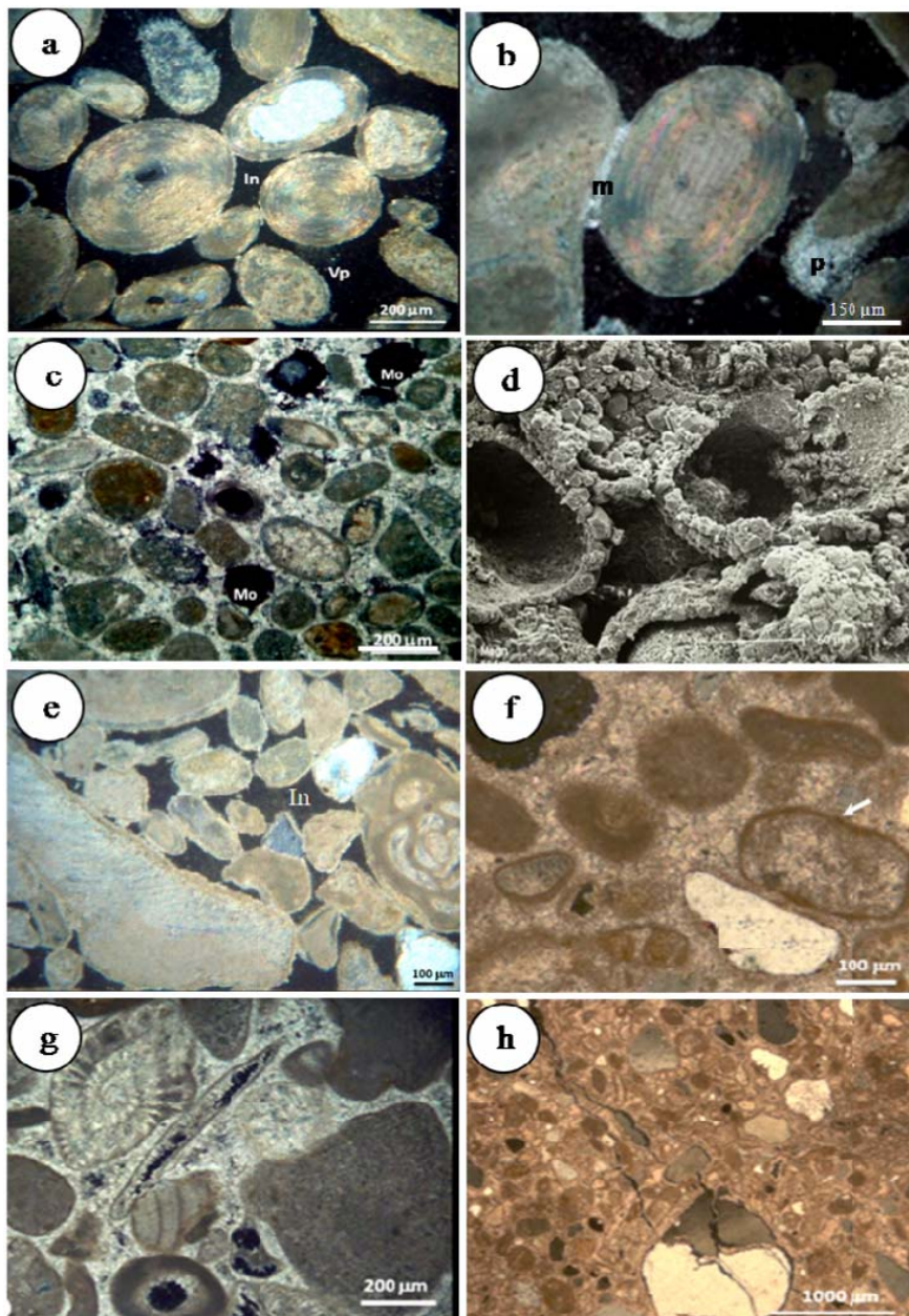
Fig. 3 Photomicrographs and SEM of the calcarenite limestones of the four ridges. The first ridge a & b: Note the dominance of ooids with high primary intergranular porosity (In), with little vadoso cement (microcrystalline cement partially coated some ooids a, meniscus (m), pendant (p) at b. The second ridge c & d: The primary intergranular porosity has been reduced by sparry calcite cement. Oomoldic (Mo) and intragranular porosities are observed. d SEM micrograph shows the leaching of the ooids, leaving micrite envelopes and forming oomolds. The third ridge e & f: Note the dominance of bioclasts and lithoclasts with the variation of porosity from very low to high with different types, and reduced by different fabrics of cements. The fourth ridge g & h: Note the highly cementation of the rock and the reduction of the porosity. Micritization of bioclasts and development of micritic envelopes are observed in the rocks of the last two ridges (arrow). Note the fracturing of the quartz grains as a result of some pressure h
