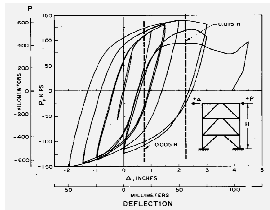
Fig. 9 Cyclic Behavior of an EBF [8]
