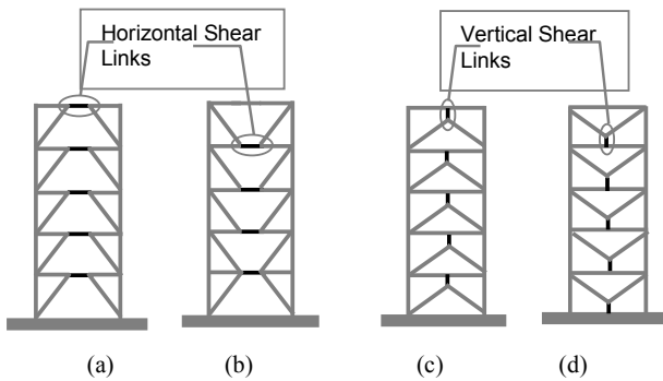
Fig. 6 Typical configuration for horizontal and vertical EBFs
