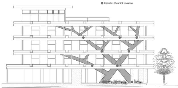
Fig. 12 Frame with shear link locations identified
