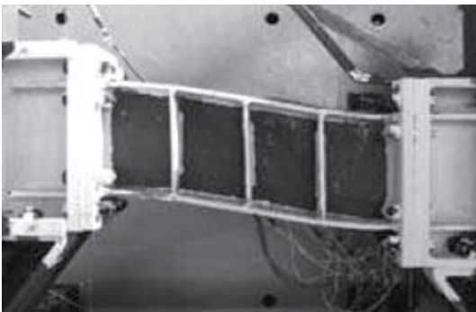
Fig. 8 (a) Shear link specimens after test [8]
