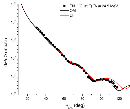
Fig. 7 Same as Fig. 5 but for energy 24.5 MeV
