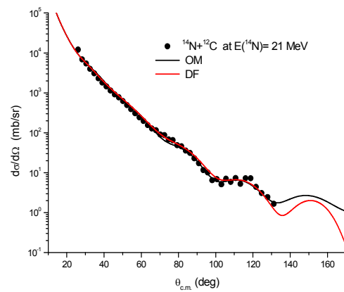
Fig. 6 Same as Fig. 5 but for energy 21 MeV
