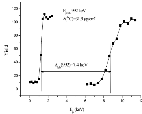
Fig. 3 The shift of the 992 keV resonance energy of the ^{27}\text{Al}(p,\gamma)^{28}\text{Si} reaction at the presence of the carbon film. The thickness of the ^{12}\text{C} target is 31.9 \mu\text{g}/\text{cm}^2
