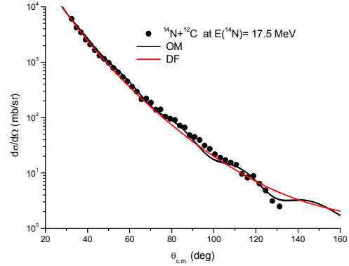
Fig. 5 Comparison between experimental and calculated differential cross section within the framework of OM and DF for ^{14}\text{N} elastically scattered by ^{12}\text{C} at energy 17.5 MeV
