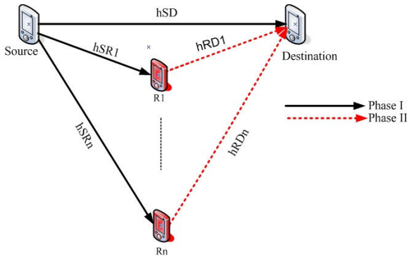
Fig. 1 Cooperative communication system
