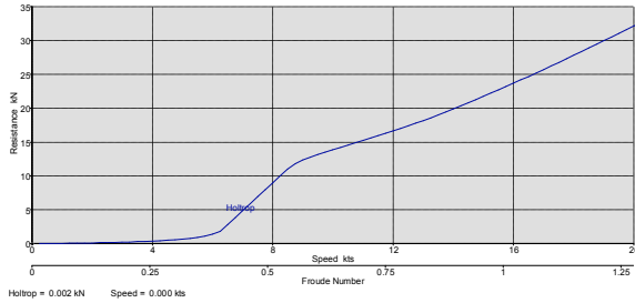
Fig. 12 Total resistance for V-shape of hull bow
