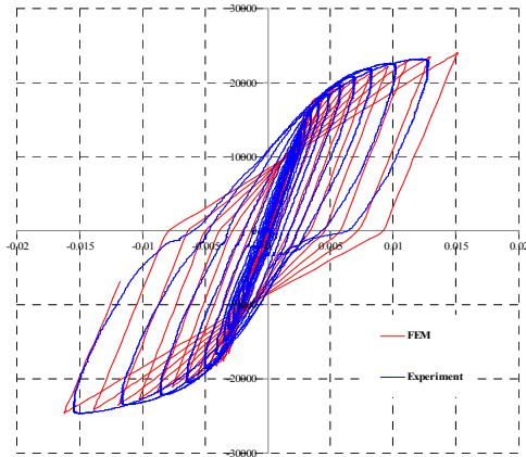
Fig. 5 Validation of T-joint system using Steel02 material
