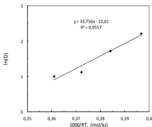
Fig. 5 \ln(D) as a function of \frac{1}{RT}
