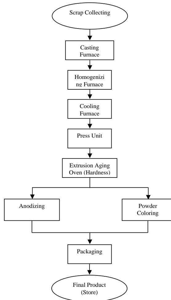
Fig. 10 Manufacturing Processes of Aluminum Sections
