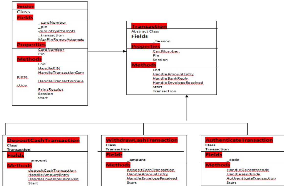
Fig. 2 Class Diagram
