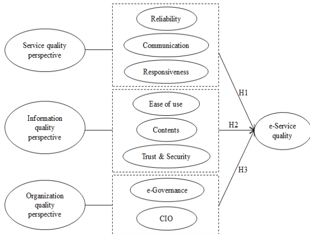
Fig. 1 Research model
