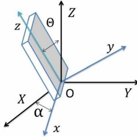
Fig. 5 The coordinates for ground and device
