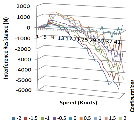
Fig. 11 Interference resistance against velocity plot for hull configurations having a constant separation and draught
