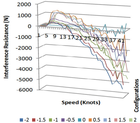
Fig. 13 Interference resistance against speed for hull configurations having a variable separation and stagger ratios with a fixed draught ratio of 0.02
