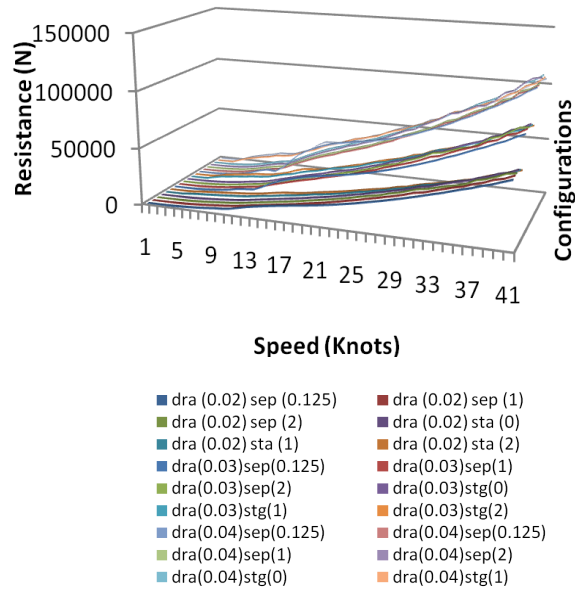
Fig. 8 Resistance against speed plot for trimarans having a variance in stagger, separation and draught ratio
