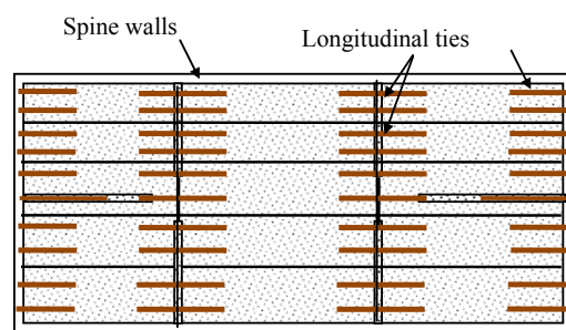
(a) Cross wall system with longitudinal ties
