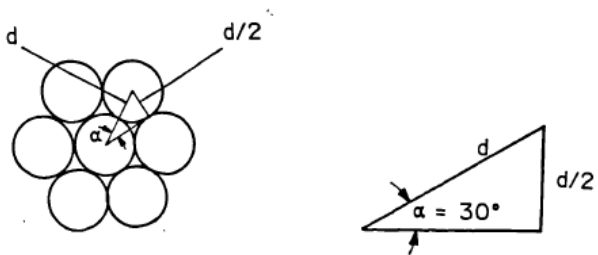
Fig. 12 The cross section of 7 wire strand
