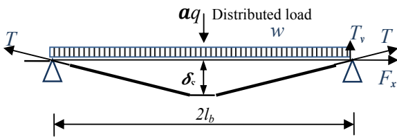
(b) Idealized catenary system
