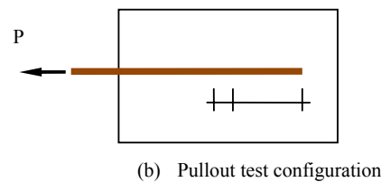
(b) Pullout test configuration
