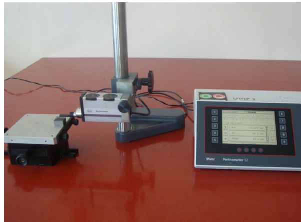
Fig. 2 Perthometer for measurement the surface roughness of the sample
