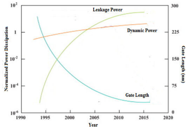
Fig. 1 Recent Power Dissipation Trends
