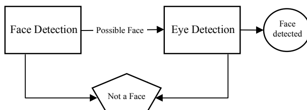
Fig. 3 Cascade of Haar feature based eye detection and face detection algorithms
