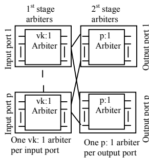
Fig. 3 Switch Allocation for ViChaR
