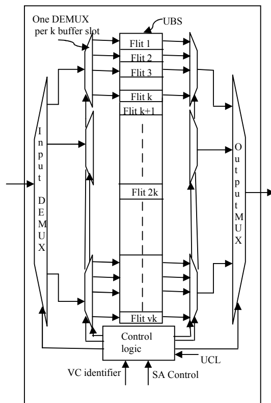
Fig. 1 Buffer architecture and allocation of ViChaR router
