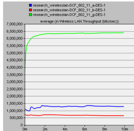
Fig. 3 Throughput of WLAN 802.11a, b and g using DCF
