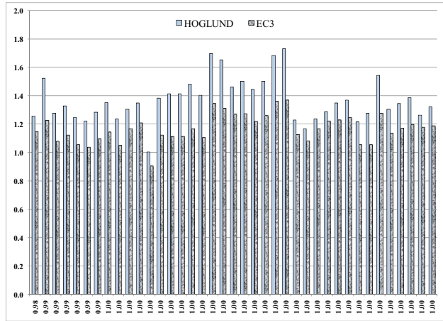
Fig. 5 Comparison between V_{exp}/V_S predicted using Höglund and EC3 for 0.98 \leq b/d \leq 1
