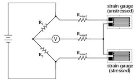
Fig. 2 Wheatstone bridge configuration of strain gauge circuit. The strain gauge labeled by 'strained' is mounted on the IC package under investigation and the one labeled by 'unstrained' is the dummy gauge for temperature compensation.
