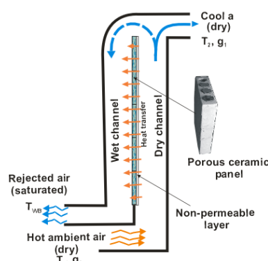
Fig. 5 A schematic of the sub-wet bulb temperature porous ceramic evaporative cooler
