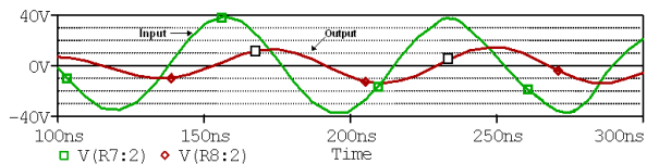
Fig. 7 Voltage indicated on the transmitter and receiver coils
