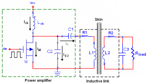
Fig. 2 Class-E power amplifier and inductive link blocks
