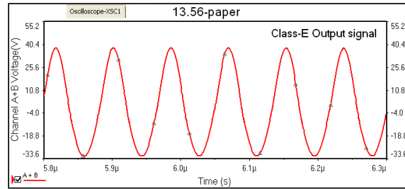
Fig. 5 The class-E output signal
