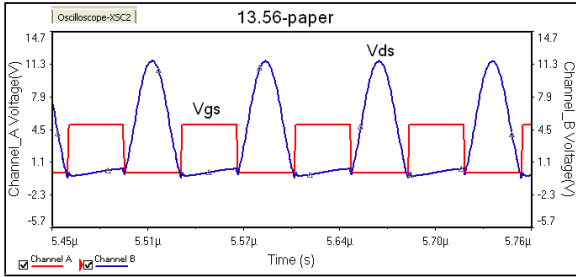
Fig. 4 Class-E performance, drain-source and gate-source in time
