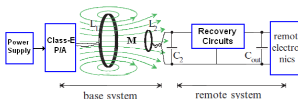
Fig. 1 Inductive power transmission block
