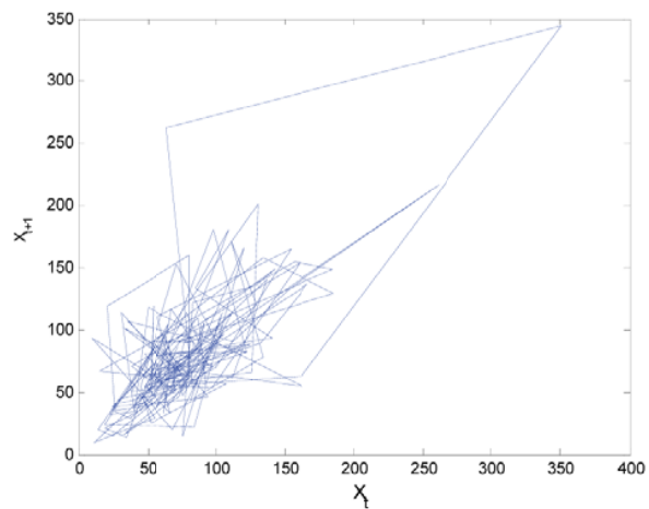
Fig. 2 Phase space
