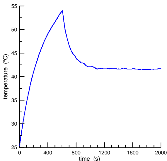
Fig. 14 Temperature versus time
