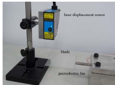
Fig. 5 Experimental equipments for blade tip displacement
