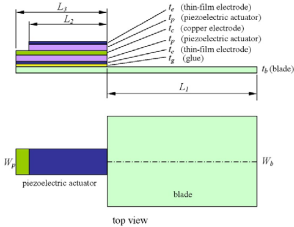
Fig. 2 Geometry of piezoelectric cooling fan
