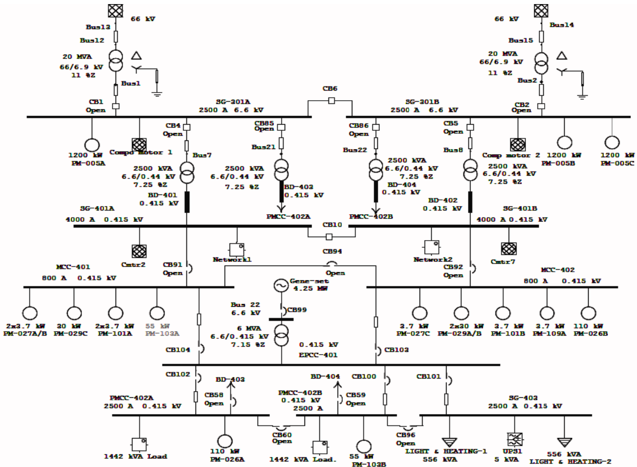
Fig. 1 Single line diagram (SLD) of OST
