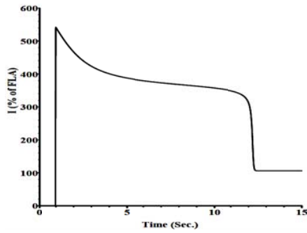
Fig. 3 Motor starting current variation with time
