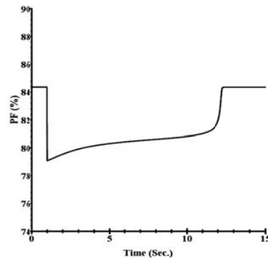
Fig. 8 Generator power factor variation during motor starting
