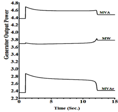
Fig. 7 Generator output power variation during motor starting
