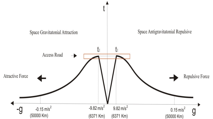
Fig. 4 Representation of the space-time terrestrial gravity
