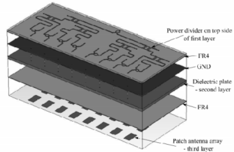
Fig. 4 Antenna structure
