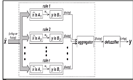
Fig. 4 Basic structure of an Inference engine
