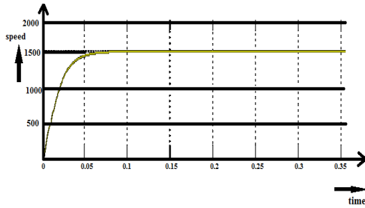
Fig. 10 Dynamic behavior of motor step response of the simplified rule base derivation
