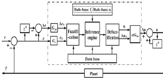
Fig. 5 Block diagram of an STFC
