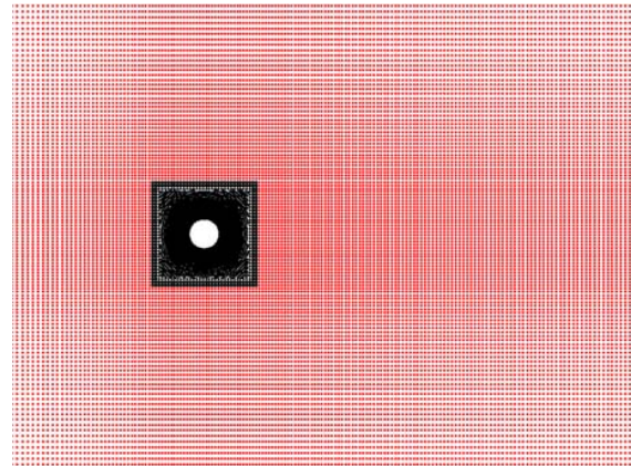
(a) Nodes in Cartesian and meshfree zones
