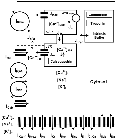
Fig. 1. Schematic diagram of the mouse model ionic currents and Ca^{2+} fluxes. Transmembrane currents are: I_{NaCa} , the fast Na^+ current, I_{CaL} , the L-type Ca^{2+} current, I_p(Ca) , the Ca^{2+} pump, I_{NaCa} , the Na^+-Ca^{2+} exchanger, I_{Kto,f} , the rapid transient outward K^+ current, I_{Kto,s} , the slow transient outward K^+ current, I_{Kr} , the rapid delayed-rectifier K^+ current (mERG), I_{Kur} , the ultra-rapid delayed-rectifier K^+ current, I_{Kss} , the steady-state non-inactivating K^+ current, I_{K1} , the time-independent K^+ current, I_{Ks} , the slow delayed-rectifier K^+ current, I_{NaK} , the Na^+-K^+ pump, and I_{Cab} and I_{Nab} , the Ca^{2+} and Na^+ background currents. I_{stim} is the external stimulation current. The Ca^{2+} fluxes within the cell are: J_{up} , uptake Ca^{2+} from the cytosol to the network sarcoplasmic reticulum (SR), J_{rel} , Ca^{2+} release from the junctional SR, J_{tr} , Ca^{2+} flux from the network to junctional SR, J_{leak} , Ca^{2+} leak from the SR to the cytosol, J_{xfer} , Ca^{2+} flux from the subspace volume to the bulk myoplasm, J_{trpn} , Ca^{2+} flux to troponin. The model includes Ca^{2+} buffering by troponin and calmodulin in the cytosol and by calsequestrin in the SR. Modified from [4].
