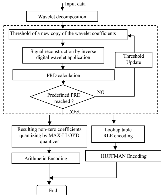
Fig. 1 Encoding Algorithm
