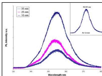
Fig. 3 The near band edge PL spectra of samples etched under different durations
