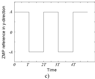
Fig. 3 Fixed ZMP references.
