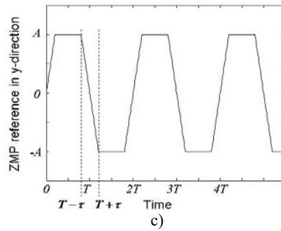
Fig. 5 Forward moving ZMP references with pre-assigned double support phases.
