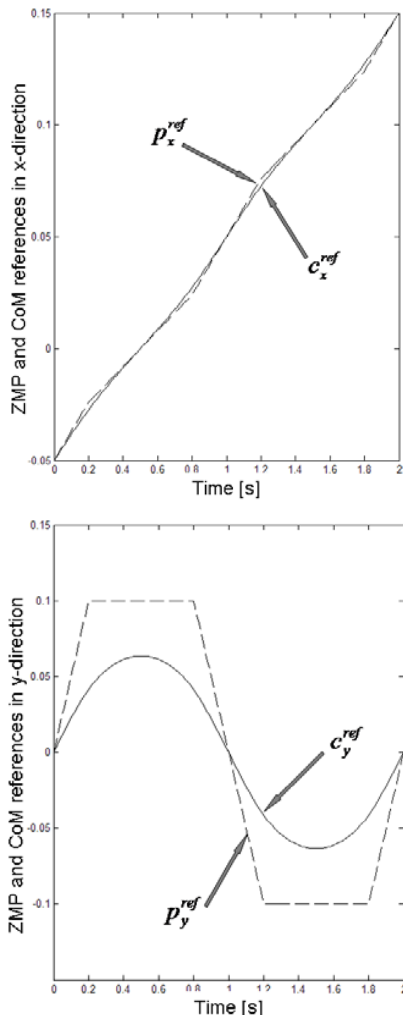
Fig. 8 x and y -direction CoM references together with the corresponding original ZMP references
