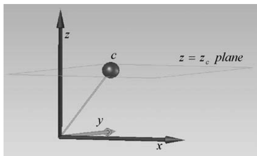
Fig. 2 The linear inverted pendulum model
