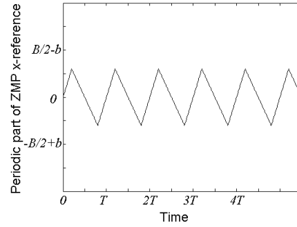
Fig. 7 p_x^{ref}(t) , the periodic part of the x -direction ZMP reference p_x^{ref}(t)
