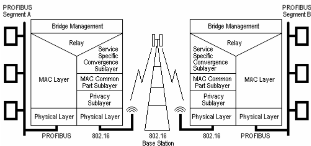
Fig. 4 Internetworking Unit Protocol Architecture
