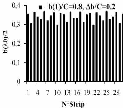
Fig. 6 (a) Normalized radiating patterns E_{\theta}/E_{\theta_{max}} (dB) for N=19 and N_{strip}=30 ( L_0 \approx 20\lambda_0 ) at f=80 GHz. (b) Sinusoidal distributions b(\lambda_0)/2 of metallic strips. \epsilon_r=2.5 , C=0.734\lambda_0 , a=0.32\lambda_0 , W=0.3307\lambda_0 , d=0.667\lambda_0 . ( \lambda_0=3.75 mm at f_0=80 GHz).
