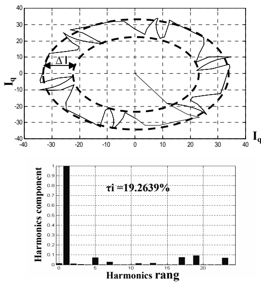
Fig.5 Current and corresponding harmonics delivered by five level inverter to an IM
