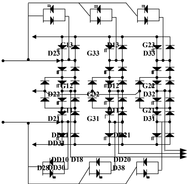
Fig. 1 Five level inverter Configuration
