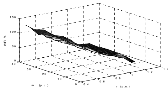
Fig.3 Harmonic spectrum voltage
