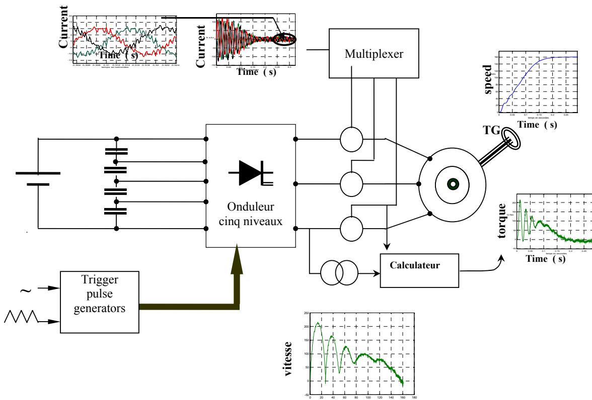
Fig.4 model simulation
