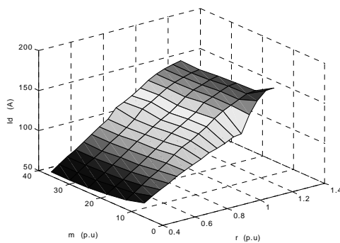
Fig. 7 Variation of the starting current of the IM according to r and m
