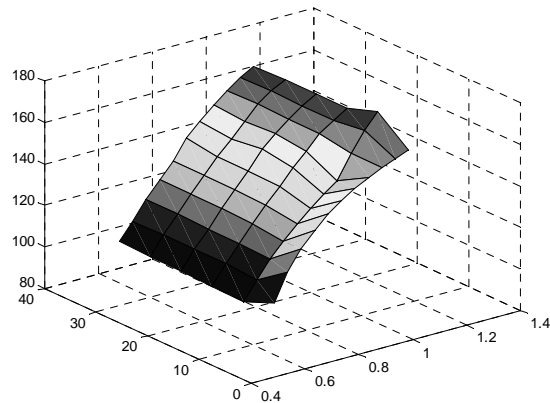
Fig. 2 Variation of RMS the inverter output voltage according to r and m
