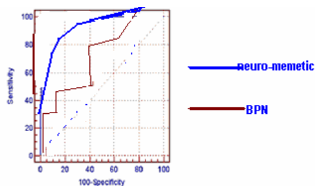
Fig. 5 Comparison of Back Propagation and Neuro-Memetic in Recognizing Numerals
