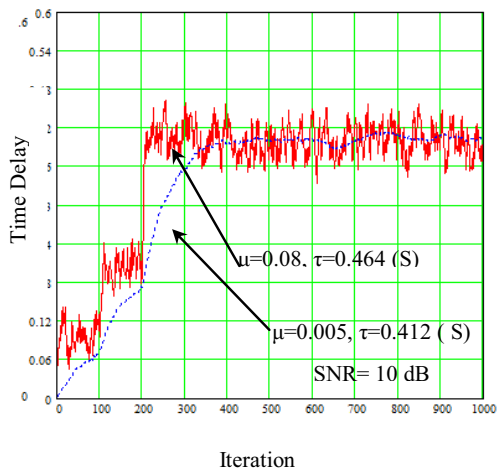
Fig. 7 The Noise and Convergence Effect on Tracking
