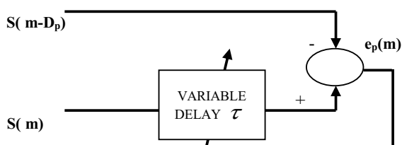
Fig. 1 Tracking time delay algorithm configuration
