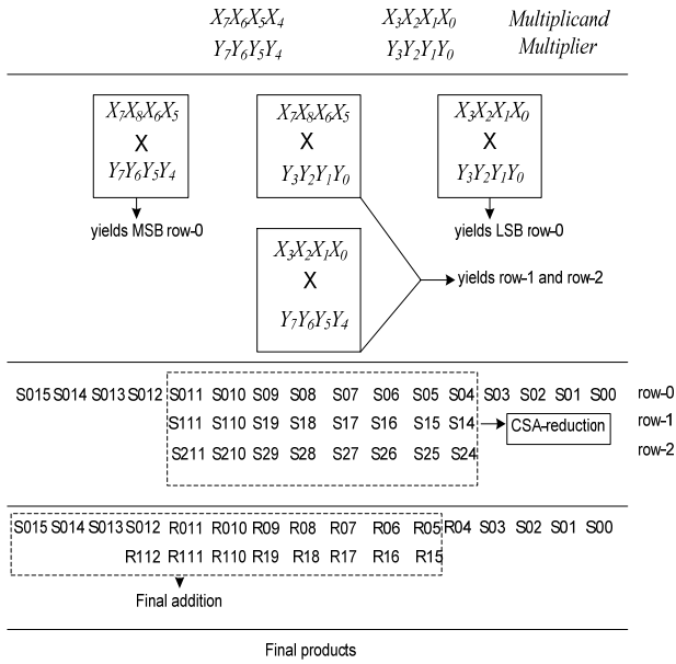
Fig. 2 8x8 proposed multiplier
