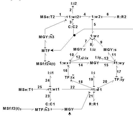
Fig. 4 Linearized bond graph
