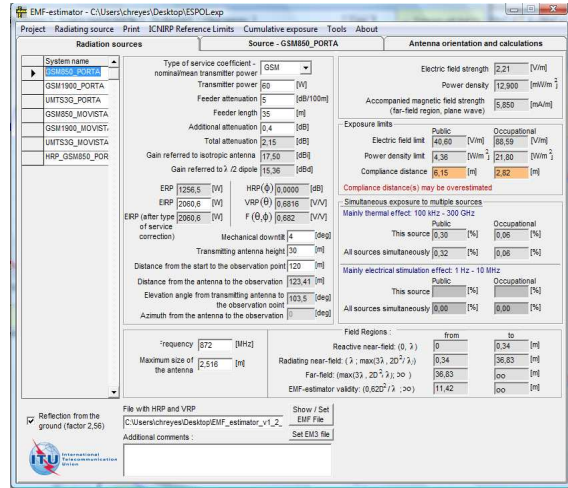
Fig. 5 Configuration of PORTA GSM 850
