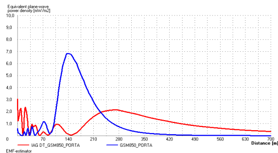
Fig. 9 Exposure levels and Increased antenna gain
