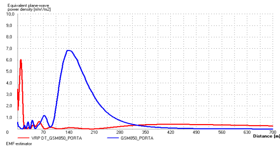
Fig. 8 Exposure levels and Decreased VRP downtilt
