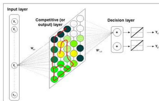
Figure 1: From left to right, the first two layers represent the general architecture of the Self Organizing Map (SOM): X_i(i=1\dots23) input corresponds to the percentage of the power spectrum of 1 band (PSSi). W_{ip}(p=1\dots23, n=1\dots25) weights from input to competitive layer. The other two layers indicate the principle of Learning Vector Quantization (LVQ)
